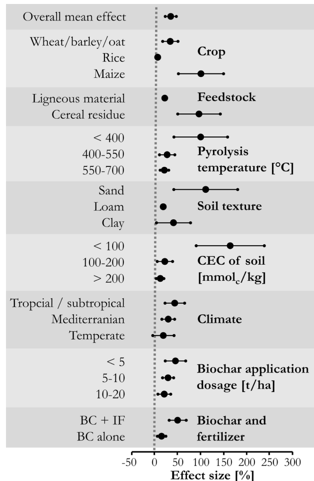
Figure 1: Impact of biochar application on crop yields in soils with different pH, soil types, climatic conditions, feedstocks, pyrolysis temperatures, and fertilizer treatment following Ye et al. (2019). CEC: cation exchange capacity; BC: biochar; BC+IF: biochar followed by inorganic fertilizer application. Dots indicate the level of impact in % relative to respective control trials. Bars indicate the 95% confidence interval. Where the left side of the error bar intersects the dotted line (zero % effect), no significant yield increase has been observed.
